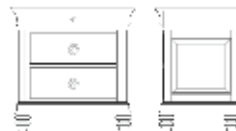
7112 Nightstand 30" x 19" x 30 1/2" H Three Drawers, Recessed Power Strip on Back Panel
