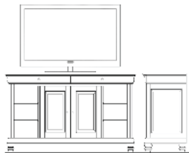
7115 Media Console 60" x 20" x 36" H Two Drawers, Two Doors, Six Adjustable Shelves, Interchangeable Wood and Glass Door Panels Interior Compartment 28" W x 23 1/2" H x 18" D Exterior Shelf Opening 10 15/16" W x 18" D Shown to Scale with 46" LCD Cable Ready Power Port
